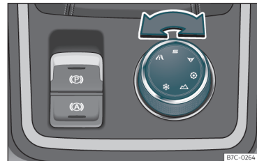
Fig. 146 Consola central: Mando rotativo (Driving Experience button).
